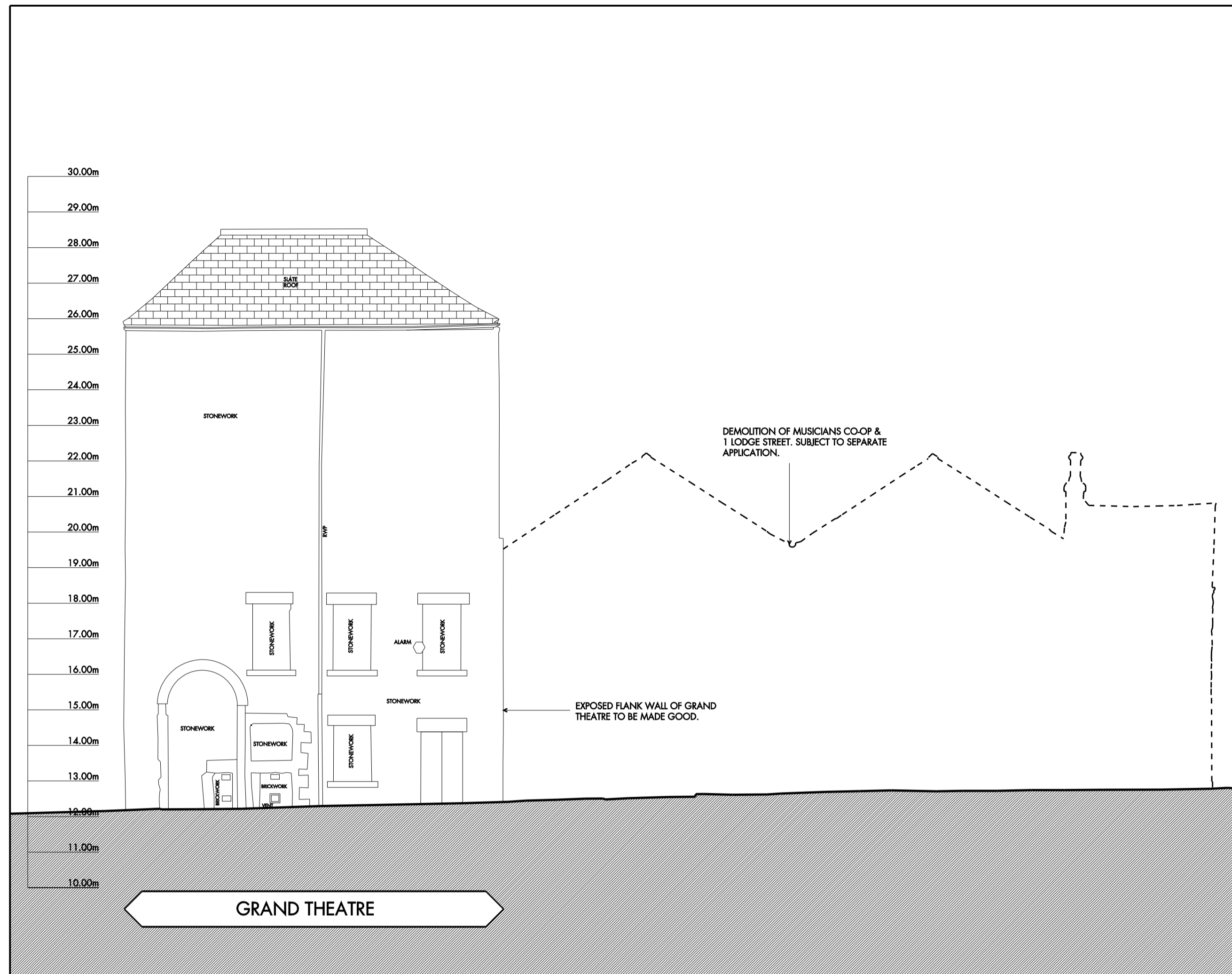
PROPOSED ELEVATION B - B
